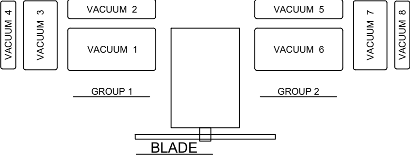
VACCUUM DIAGRAM
