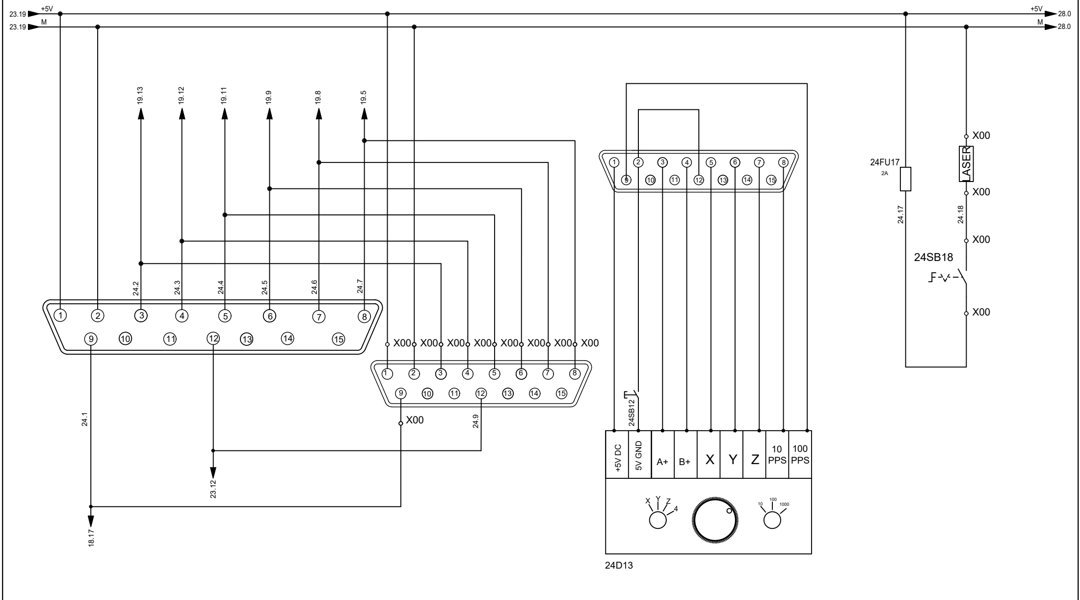
9 PIN CONNECTOR IN BOX FOR REMOTE 9 PIN CONNECTOR IN HEAD FOR REMOTE REMOTE CONTROL LASER
